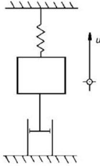
Figure 1 Mass–spring–damper system.
