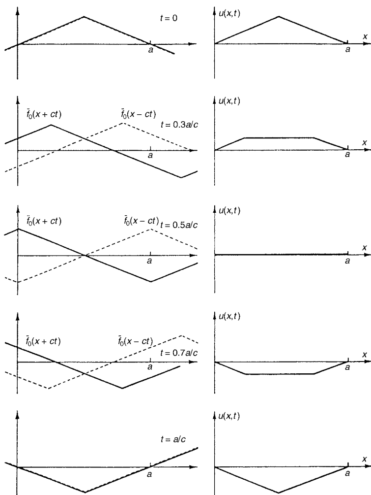
Figure 3 On the left are the graphs of \bar{f}_0(x+ct) (solid) and \bar{f}_0(x-ct) (dashed) for the given value of ct . On the right is the graph of u(x,t) for 0 < x < a , made by averaging the graphs on the left.
